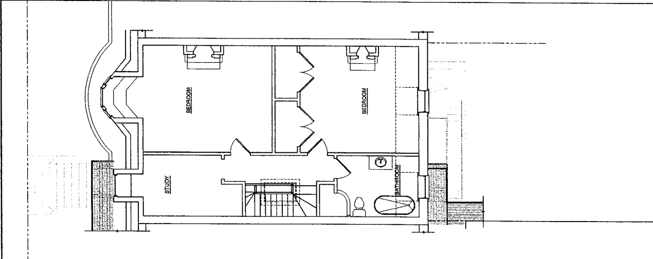
EXISTING FOURTH FLOOR PLAN SCALE: 1/4" = 1'-0"
