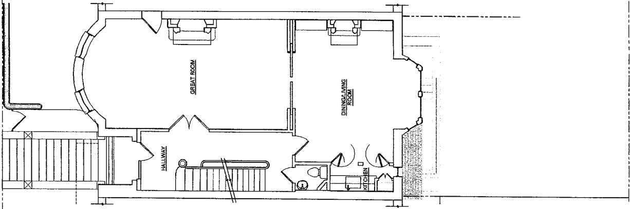
EXISTING FIRST FLOOR PLAN | SCALE: 1/4" = 1'-0" | 1
